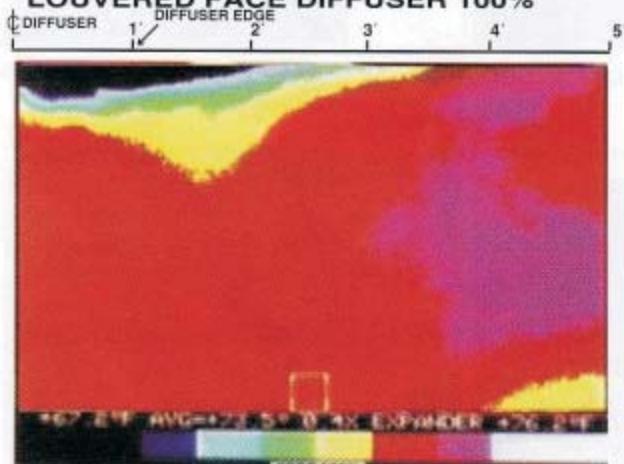
PERFORATED DIFFUSER 100%
